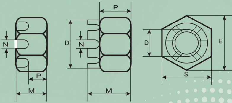
Form A Up to d=M10
